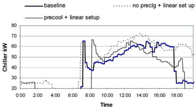
Figure 5 Effects of night pre-cooling on second day cooling load – warm days, CSSC.
