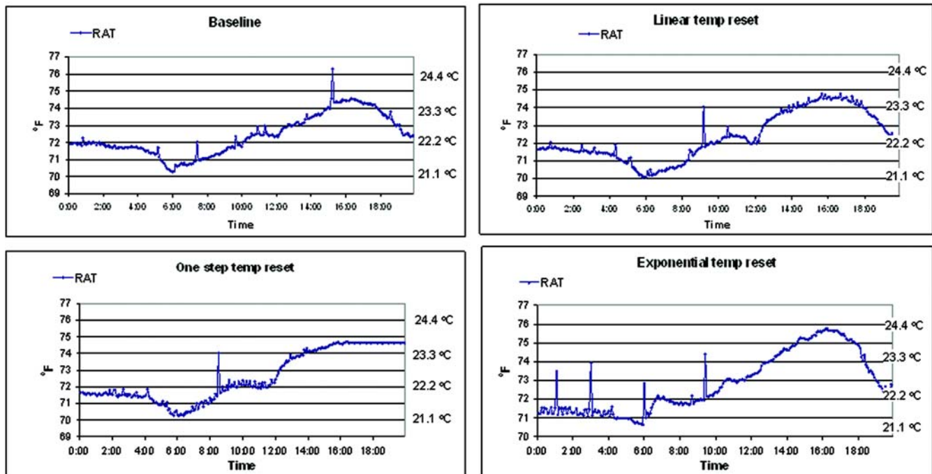
Figure 11 Comparison of return air temperatures with exponential temperature adjustment.
