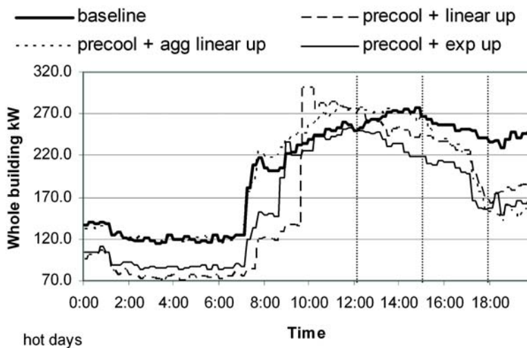
Figure 4 Effects of night pre-cooling on upcoming day cooling load – warm days, CSSC.
