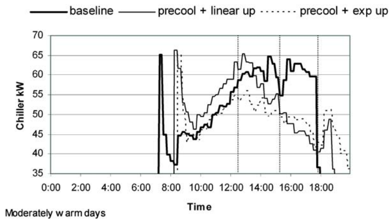
Figure 3 Cooling power reduction on pre-cooling test days – cool days, CSSC.
