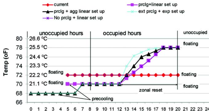
Figure 2 Cooling and demand shed strategies, CSSC.
