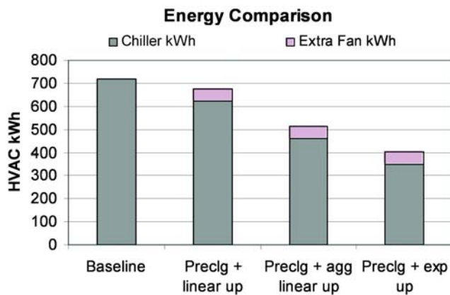
Figure 7 Energy usage of pre-cooling strategies, CSSC.
