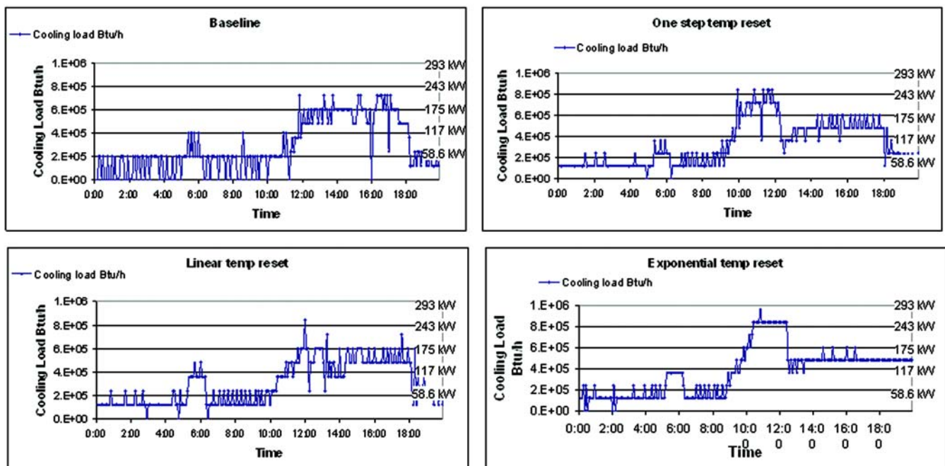
Figure 10 Comparison of different temperature reset strategies, OSF.
